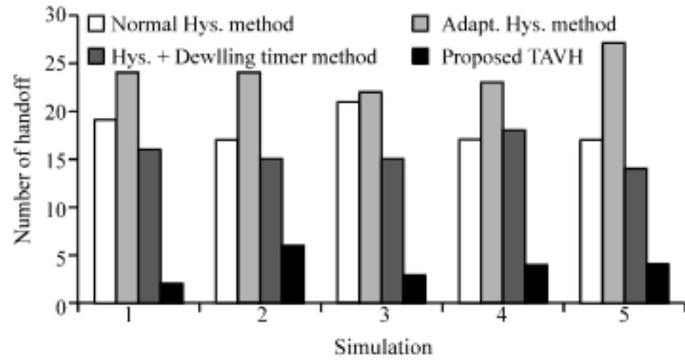
Fig. 8: Handoff failure for each method
