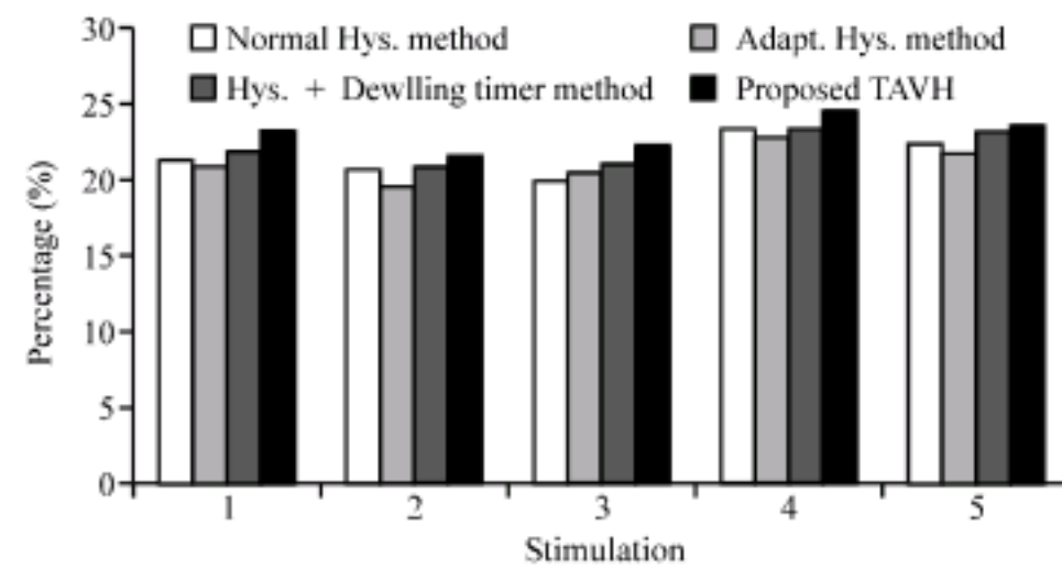
Fig. 13: Service time percentage of 3GPP for each method
