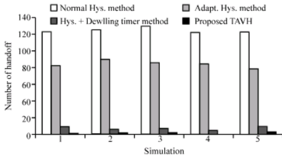
Fig. 9: False handoff for each method
