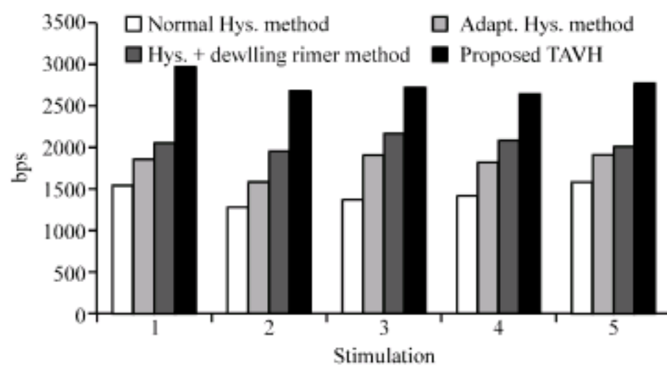
Fig. 11: Total average throughput for each method
