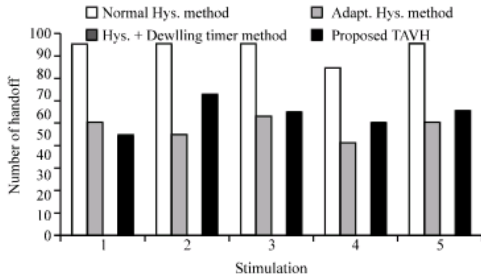
Fig. 10: Ping-pong handoff for each method
