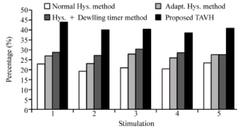
Fig. 14: Service time percentage of WiMAX for each method
