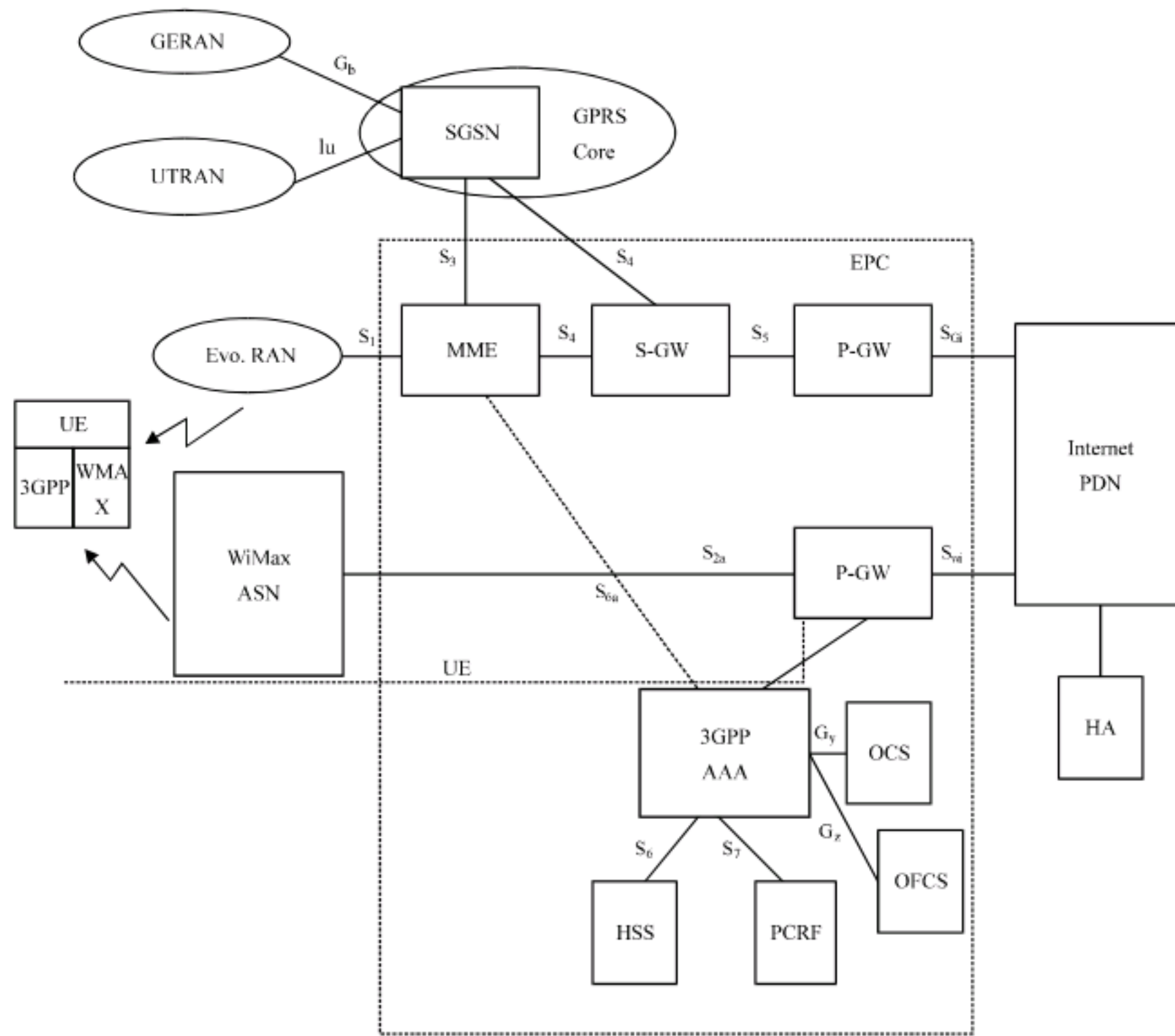
Fig. 2: Network architecture for WiMAX and 3GPP interworking
